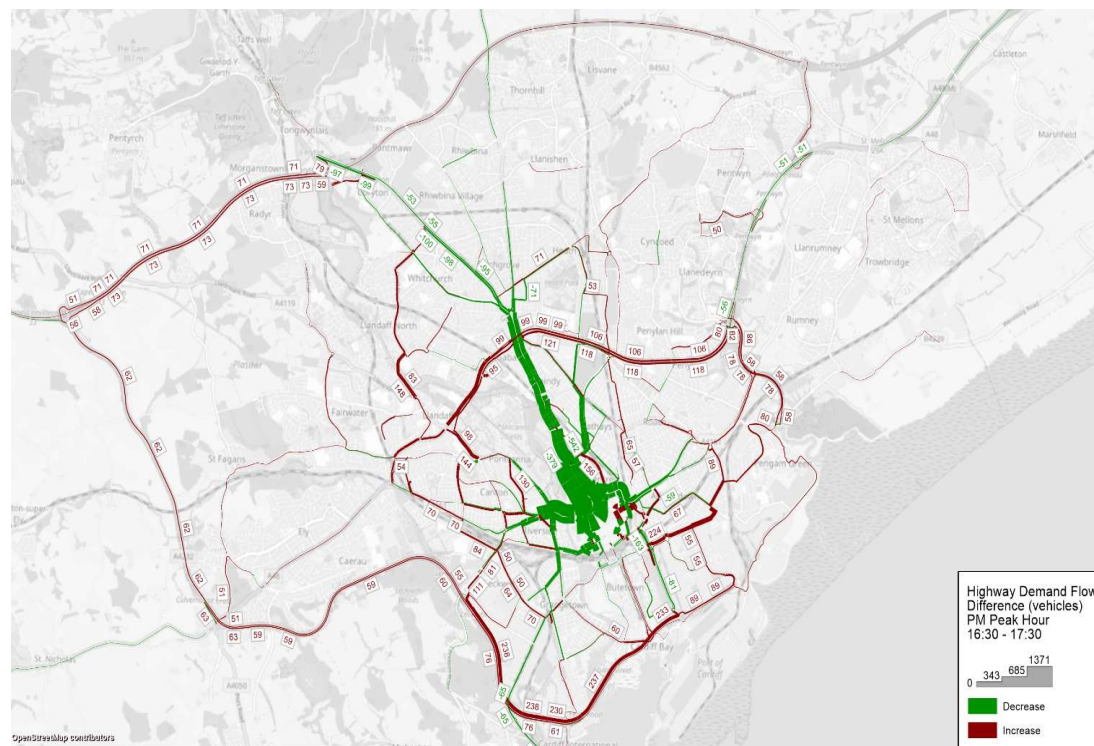
Option 2– Bus Gate pm Peak Flows
